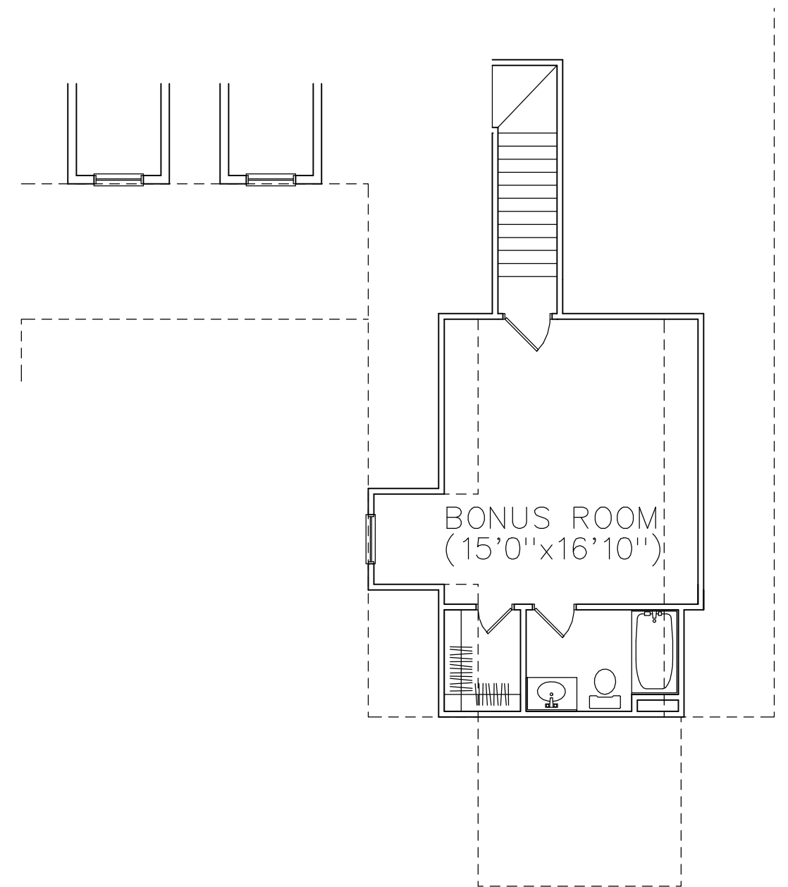
BONUS ROOM FLOOR PLAN
